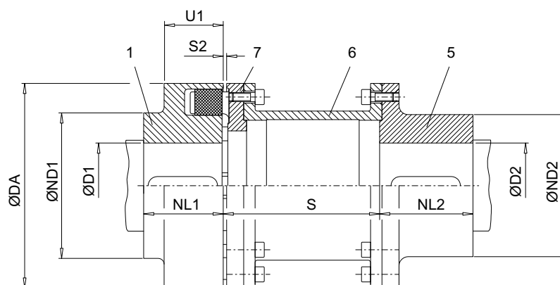
Image A-1: Type H
