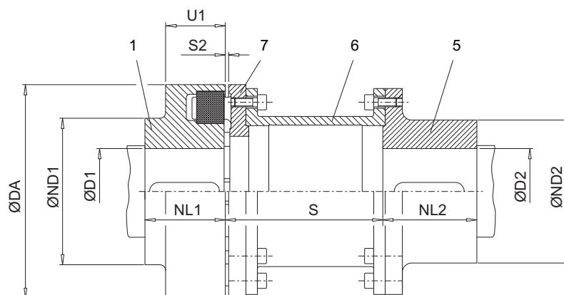
Image A-2: Type HDS
